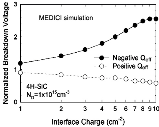
Fig. 8. Breakdown voltage change as a function of the radiation-induced interface charge density.
